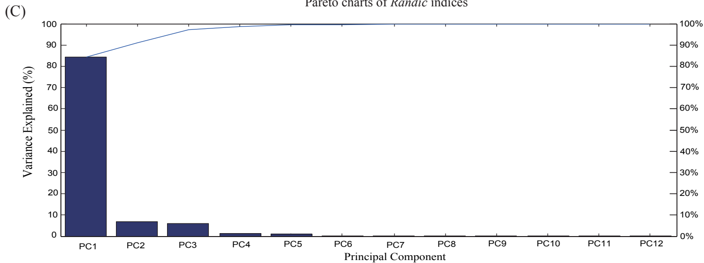
Pareto charts of Randić indices
