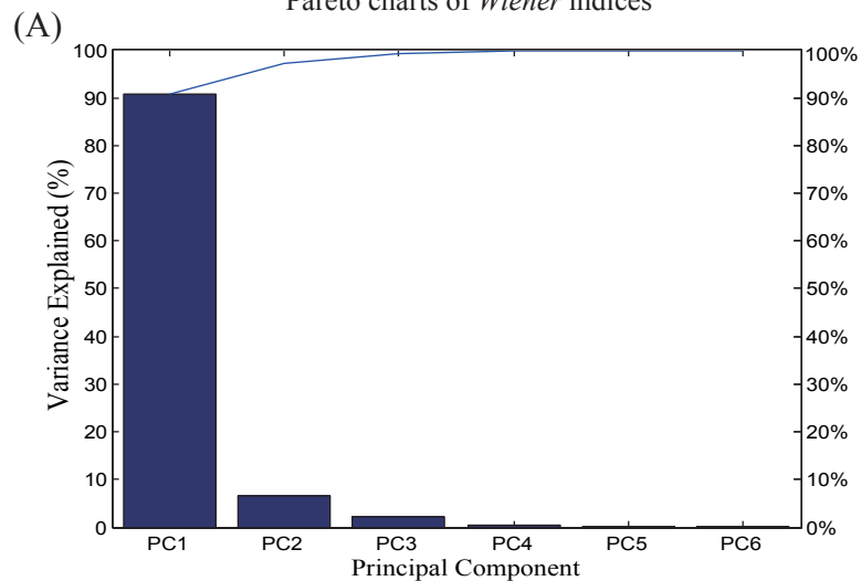
Pareto charts of Wiener indices
