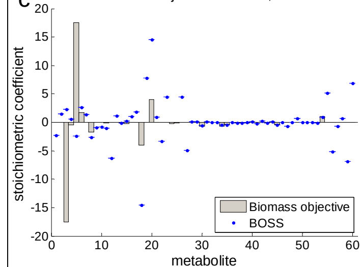
BOSS-derived Objective Function, Noise=15%
