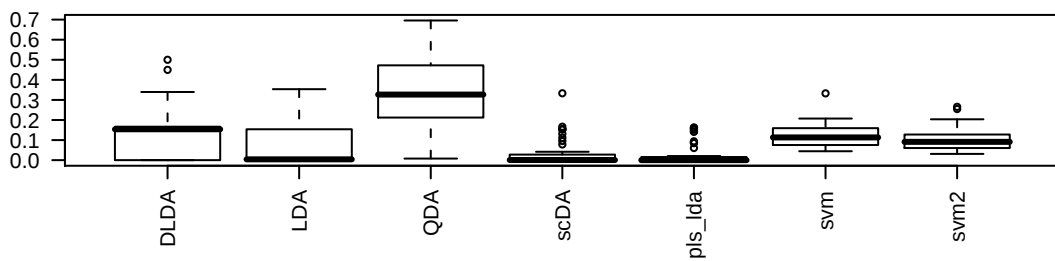
brier score
