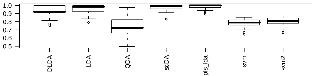
average probability
