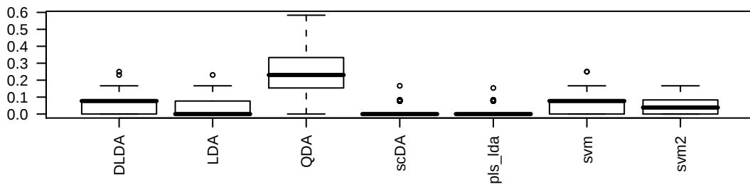
misclassification
