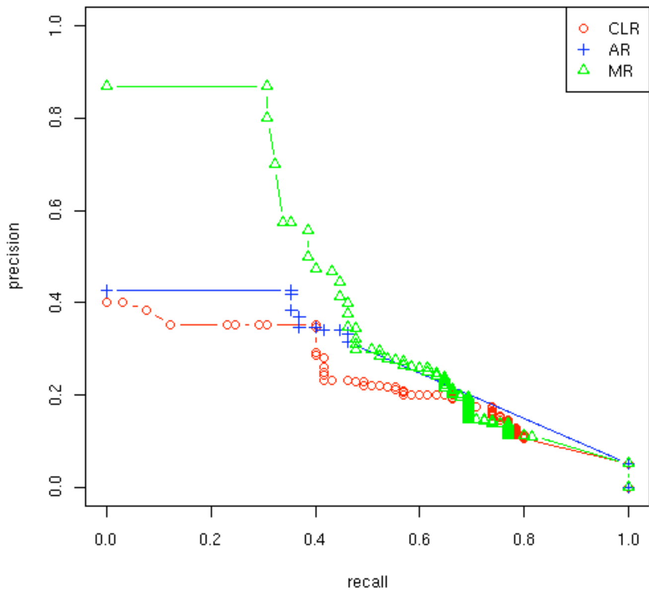
PR-Curve
