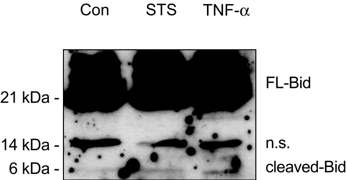
Figure 1 B: long exposure
