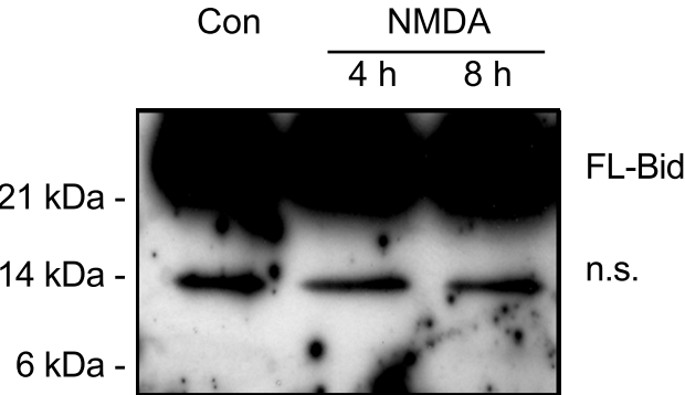
Figure 1 C: long exposure
