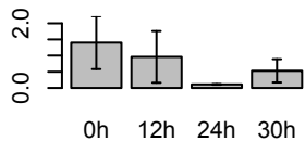
GgaAffx.4101.1.S1_at (LOC423800)
