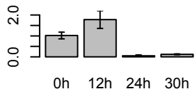
GgaAffx.11175.1.S1_at (LOC431636)
