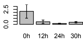
GgaAffx.4973.2.S1_s_at (LOC423163)
