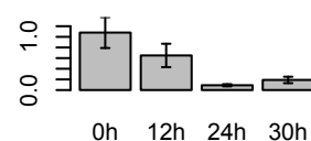
GgaAffx.2367.1.S1_at (NA)
