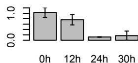
GgaAffx.21832.1.S1_s_at (FGF 13)
