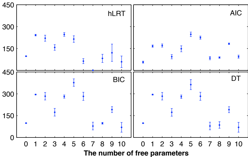
Model biases (models are classified into 11 categories)
