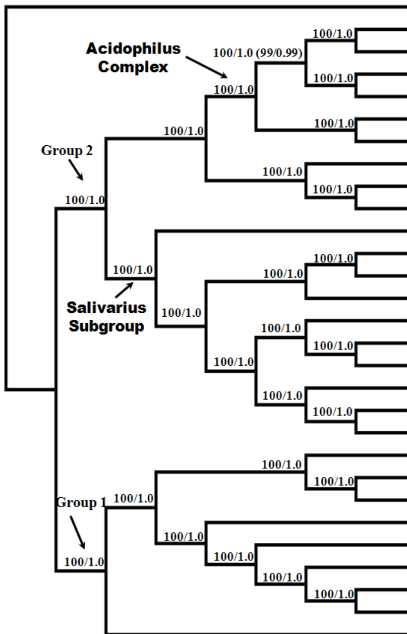
(The combined tree of 232 genes )
