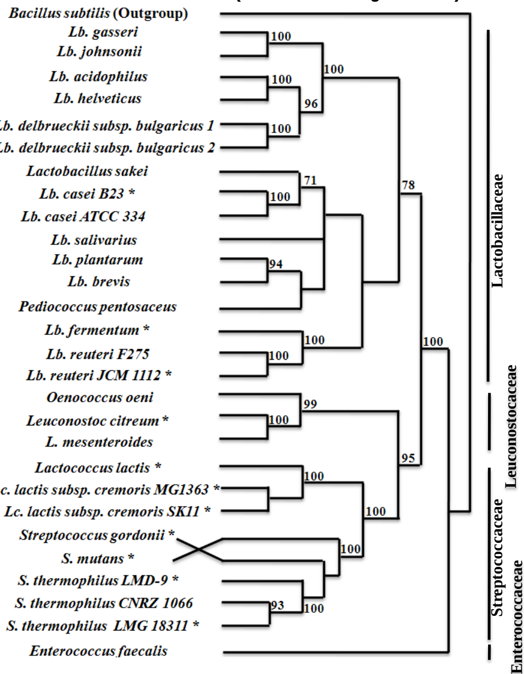
(The 16S rRNA gene tree)
