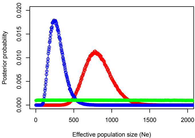
Ne, autosomes
