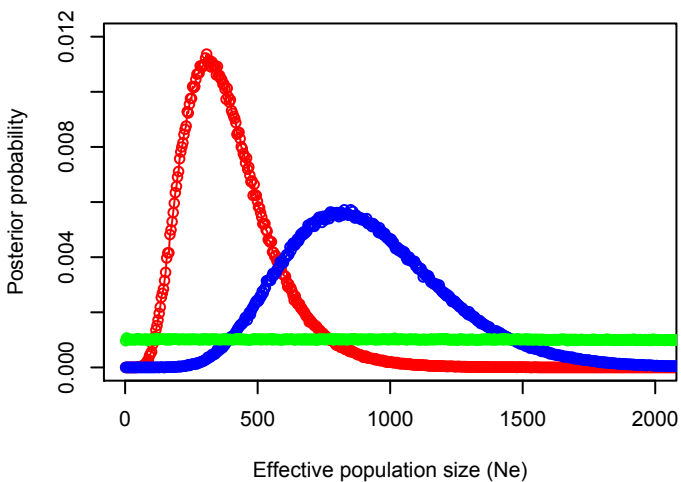
Ne, Z-chromosome
