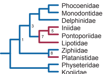
S) Yan et al. 2005 Bayes, ML: mt genome
