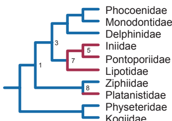
Z) Slater et al. 2010 Bayes: 1 mt gene+mt genome
