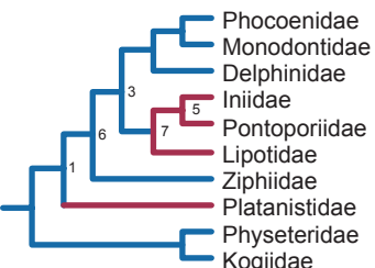
V) McGowen et al. 2009 Bayes, ML: 45 nu genes+mt genome+SINES
