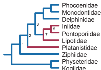
U) Agnarsson and May-Collado 2008 Bayes: 1 mt gene
