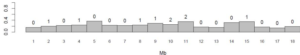
CB4856 SNP rate per Mb for Chromosome X (Number of hotspots on top of bars)
