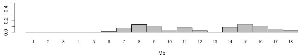
CB4858 SNP rate per Mb for Chromosome X
