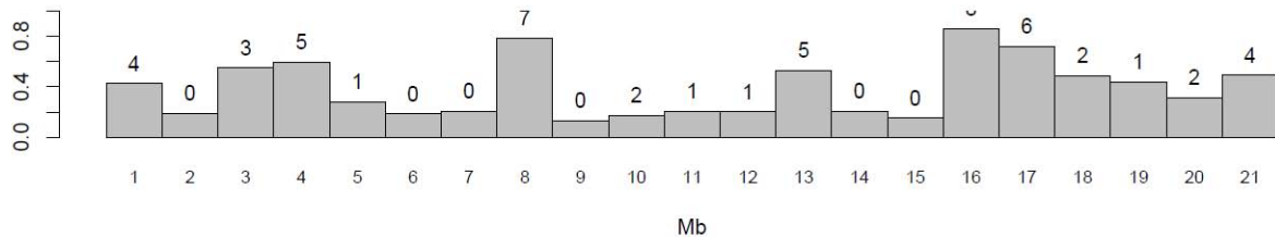
CB4856 SNP rate per Mb for Chromosome V (Number of hotspots on top of bars)
