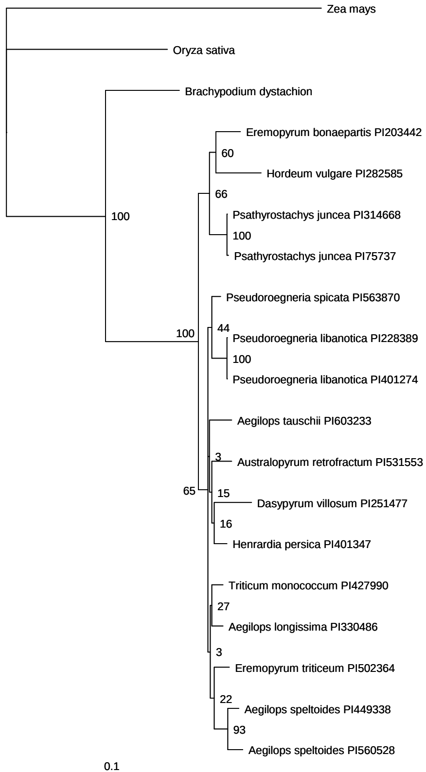
Figure S14. Phylogenetic tree inferred with LOC_Os01g60230 sequences. Values in nodes are bootstrap values.
