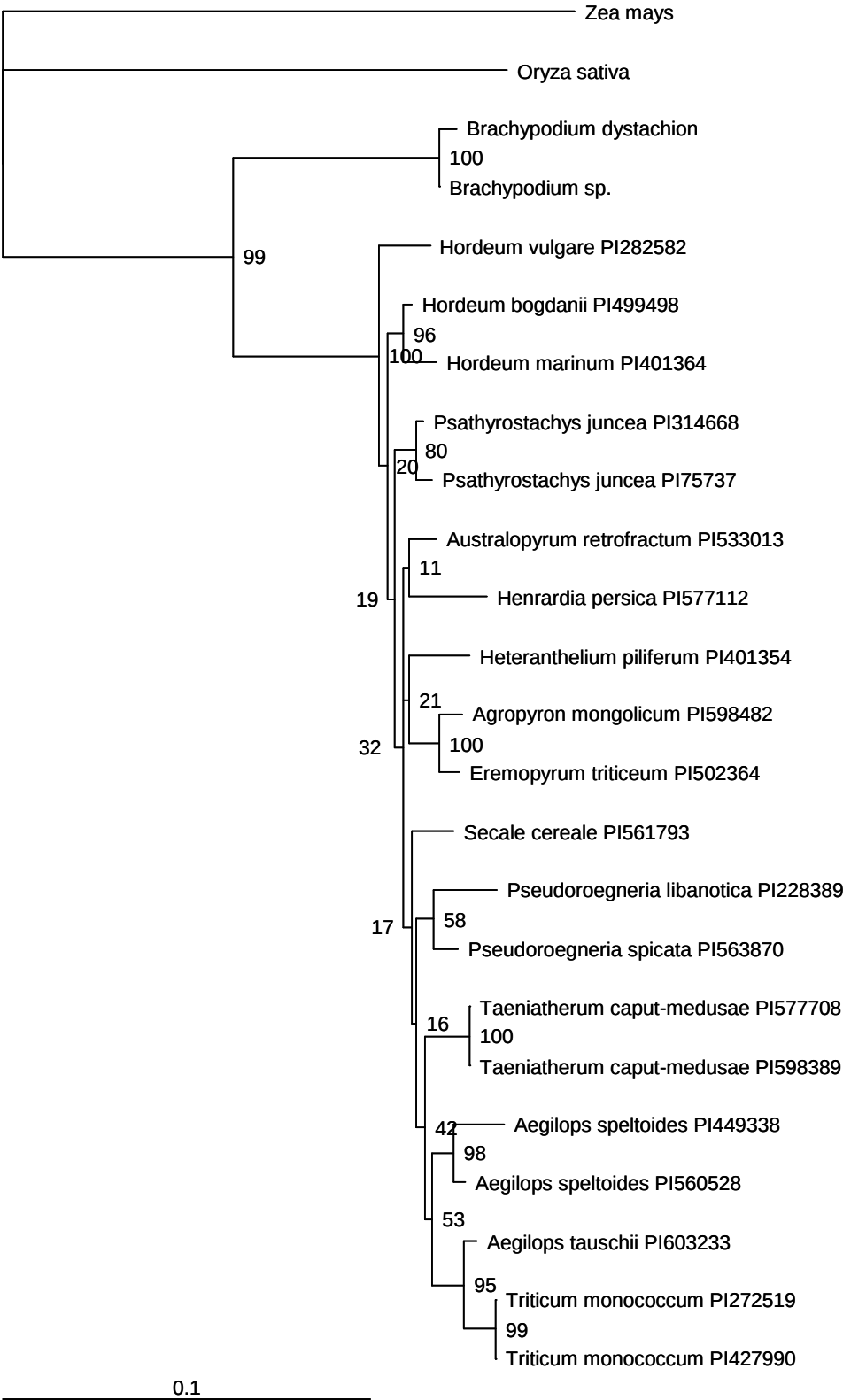
Figure S15. Phylogenetic tree inferred with LOC_Os01g61720 sequences. Values in nodes are bootstrap values.
