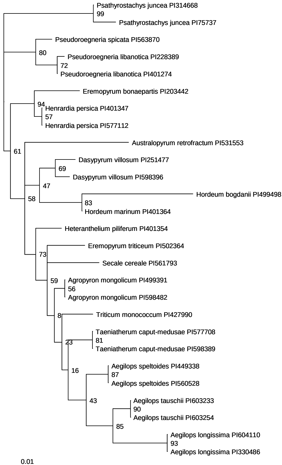
Figure S22. Phylogenetic tree inferred with eIFiso4E sequences. Values in nodes are bootstrap values.
