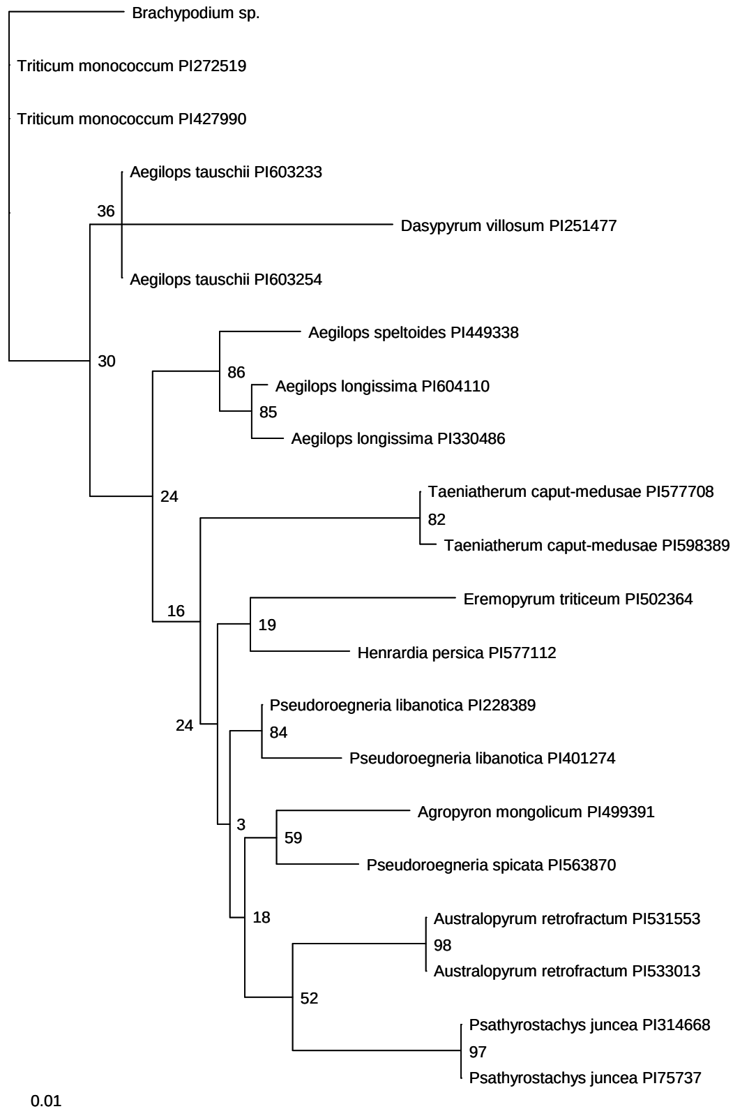
Figure S24. Phylogenetic tree inferred with PinA sequences. Values in nodes are bootstrap values.
