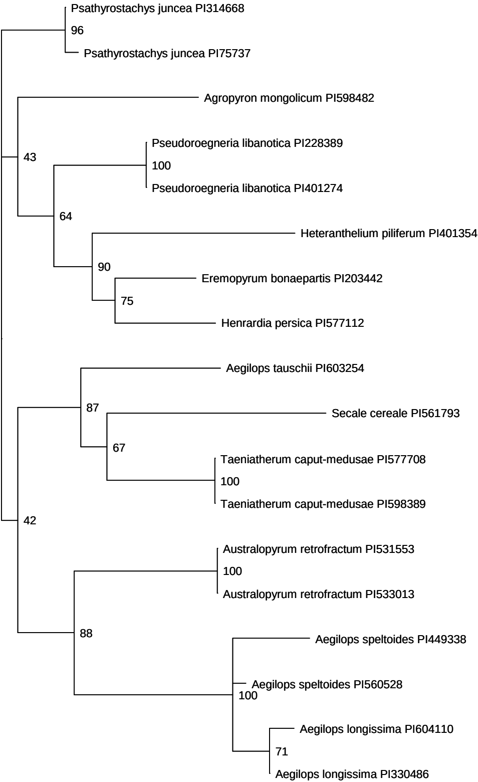
Figure S25. Phylogenetic tree inferred with PinB sequences. Values in nodes are bootstrap values.
