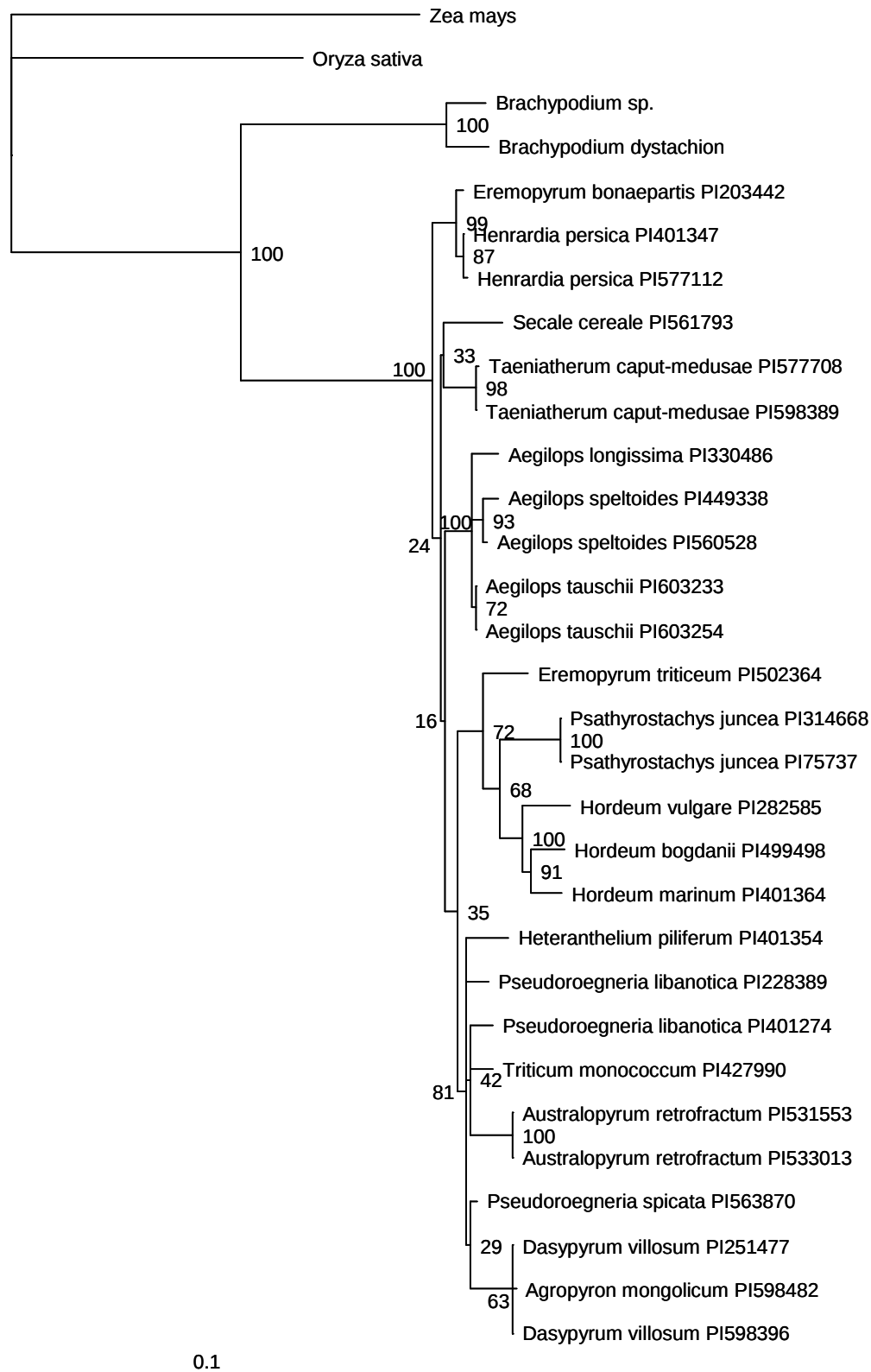
Figure S3. Phylogenetic tree inferred with LOC_Os01g11070 sequences. Values in nodes are bootstrap values.
