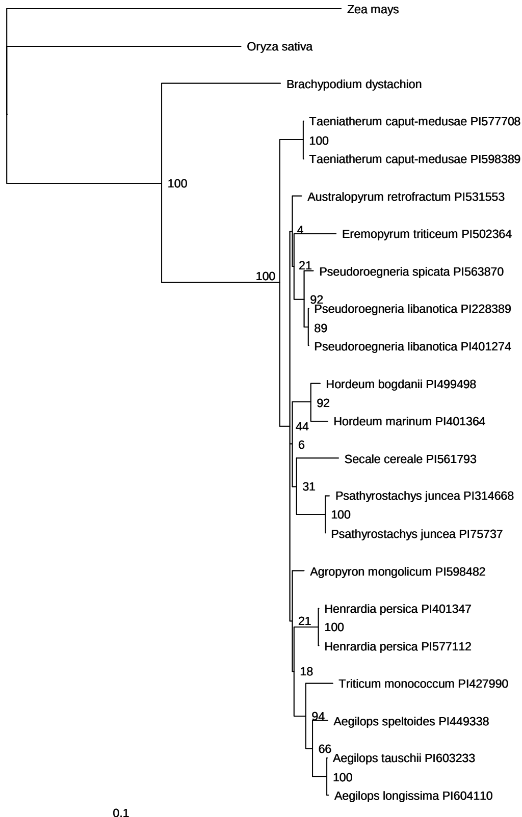
Figure S8. Phylogenetic tree inferred with LOC_Os01g37560 sequences. Values in nodes are bootstrap values.
