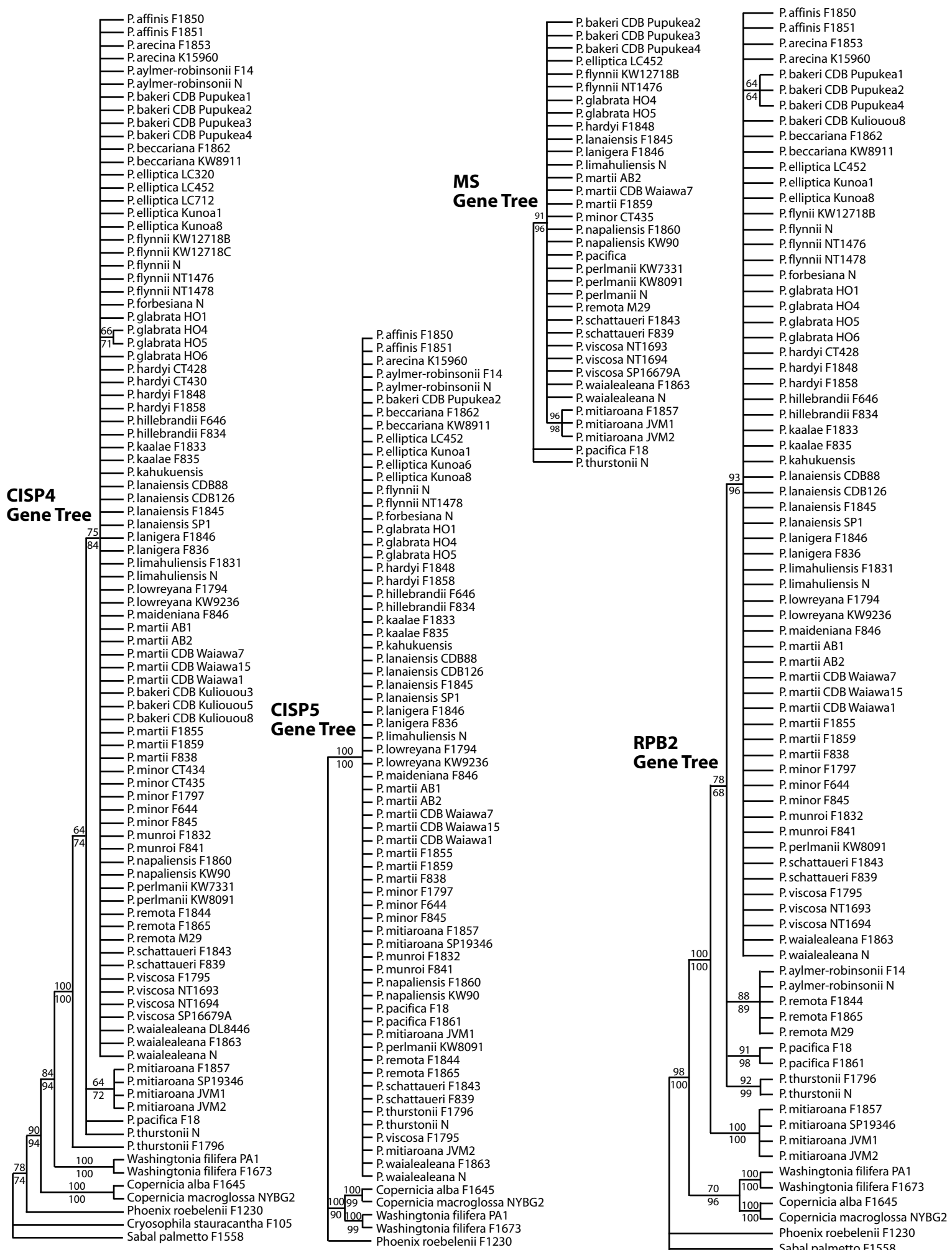
Supplemental Figure 3. The individual nuclear gene trees estimated for Pritchardia species delimitation as shown in the parsimony strict consensus with parsimony jackknife values above and likelihood bootstrap values below each branch.
