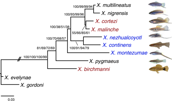
(c) mtDNA and nuDNA combined tree
