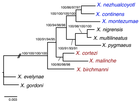
(c) mtDNA and nuDNA combined tree
