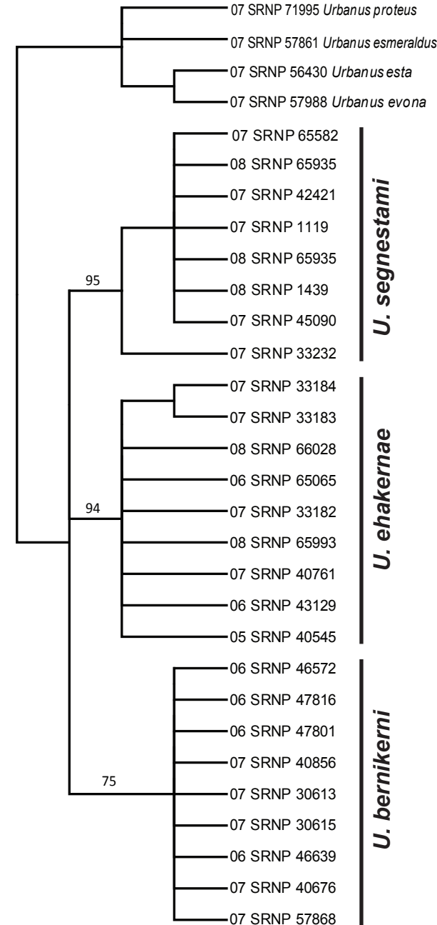
(c) EF1a
