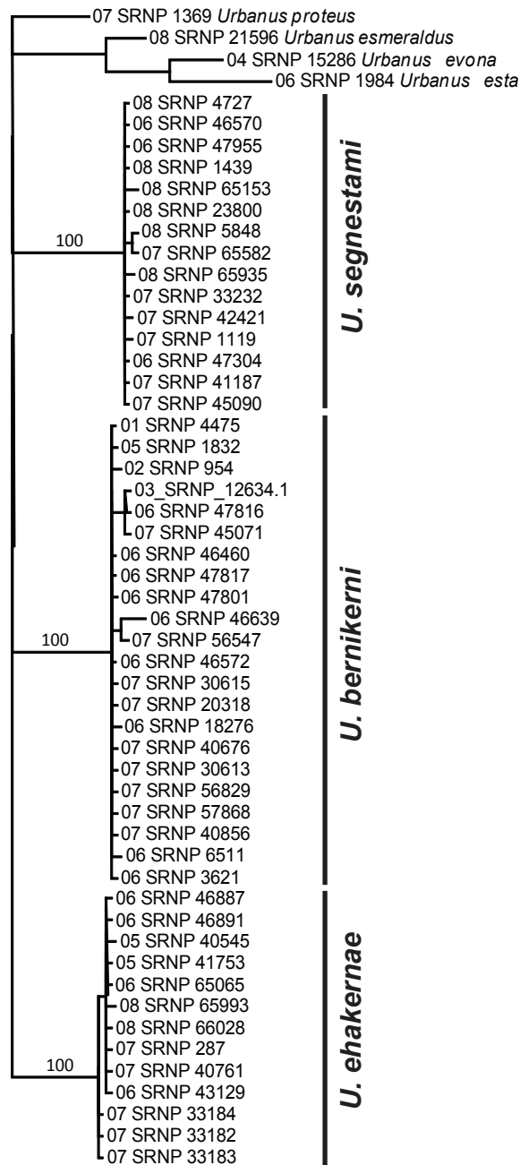
(b) cytb
