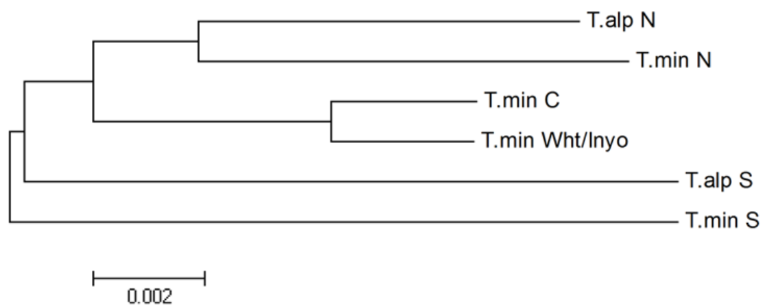
Figure S5. NJ tree of the relationships among geographic groups of T. alpinus and T. minimus based on the average number of nucleotide substitutions per site (Dxy, Nei 1987) at cyt b .
