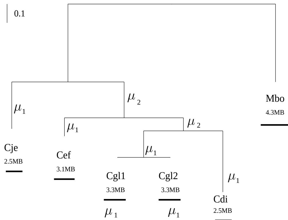
Figure S.4: An alternative topology of the concatenated genes. The insertion/deletion rates on external branches and internal branches were studied.
