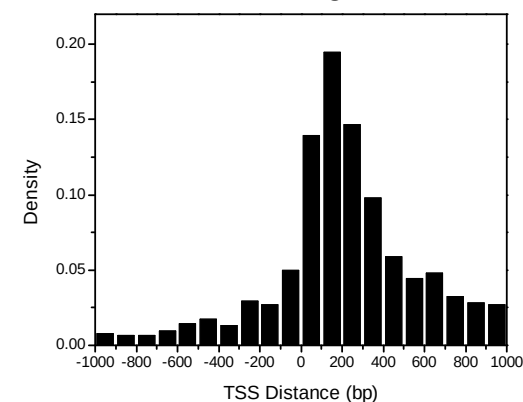
C.elegans
