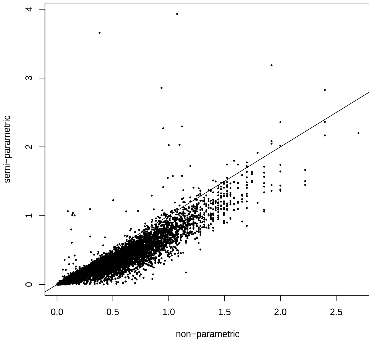
P-Values for Conditional Independence Test
