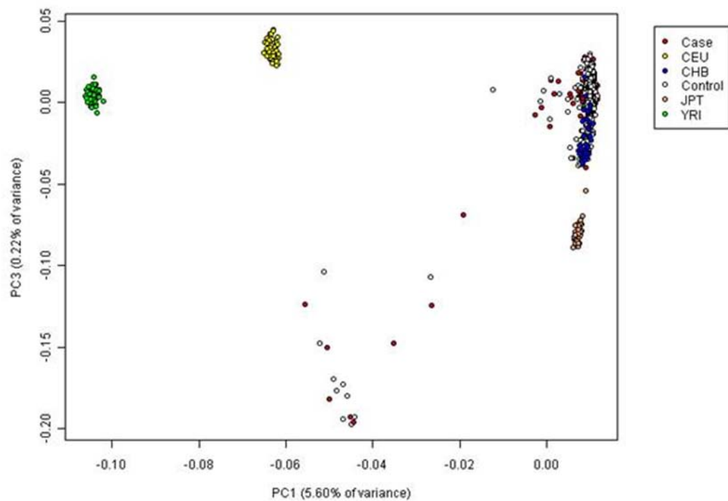
(b) PC1 vs PC3 (1028 Samples + 206 HapMap Samples)
