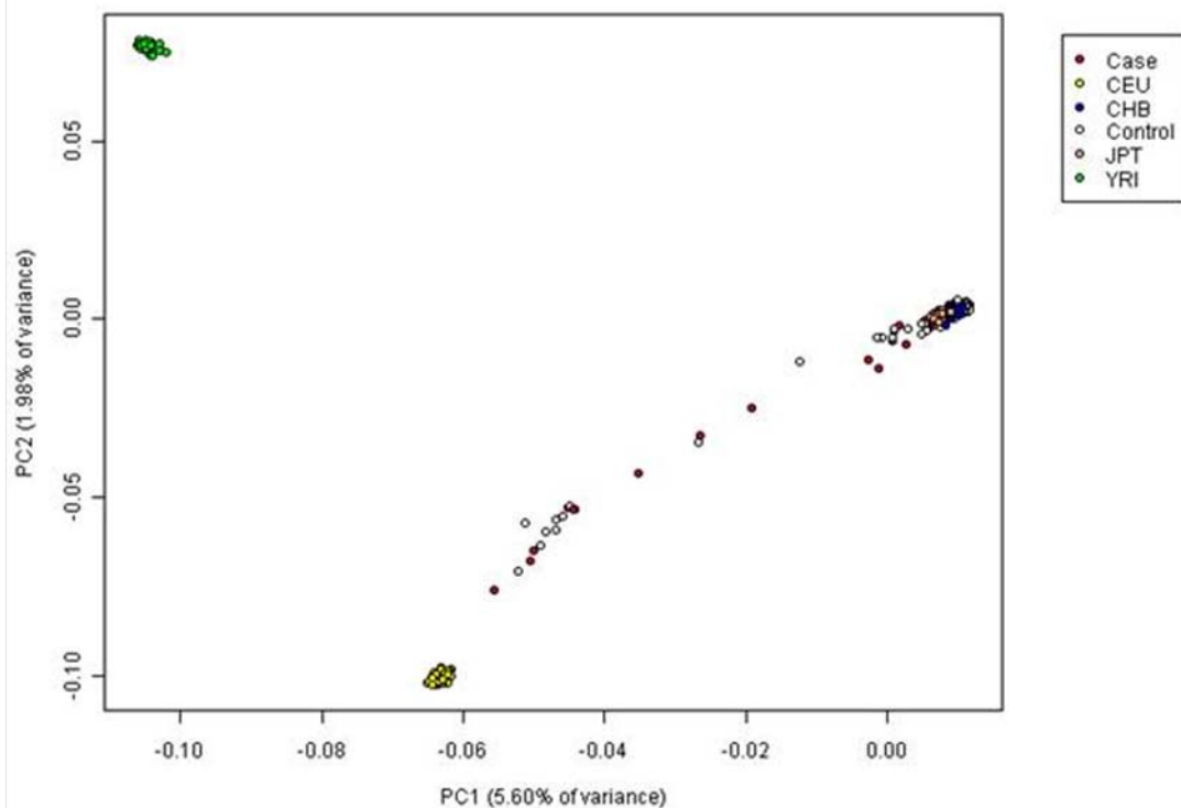
(a) PC1 vs PC2 (1028 Samples + 206 HapMap Samples)
