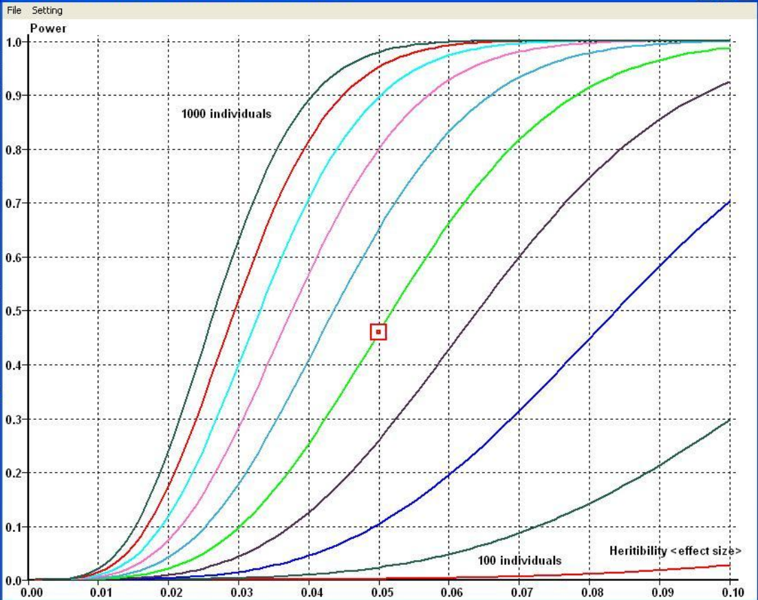
Power Curves of various individuals under different effect size
