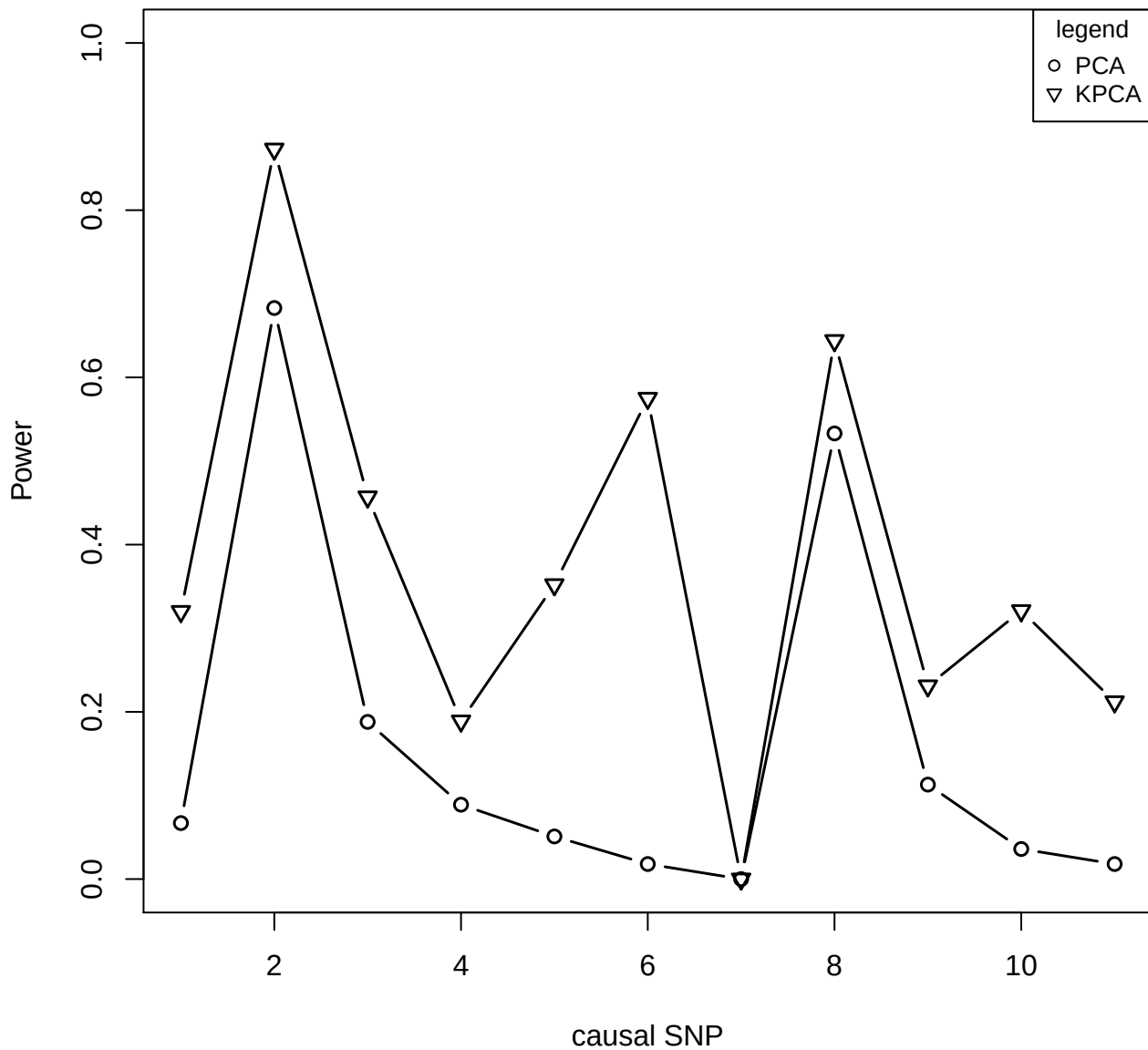
Power for RR=1.3 and sample_size=3000
