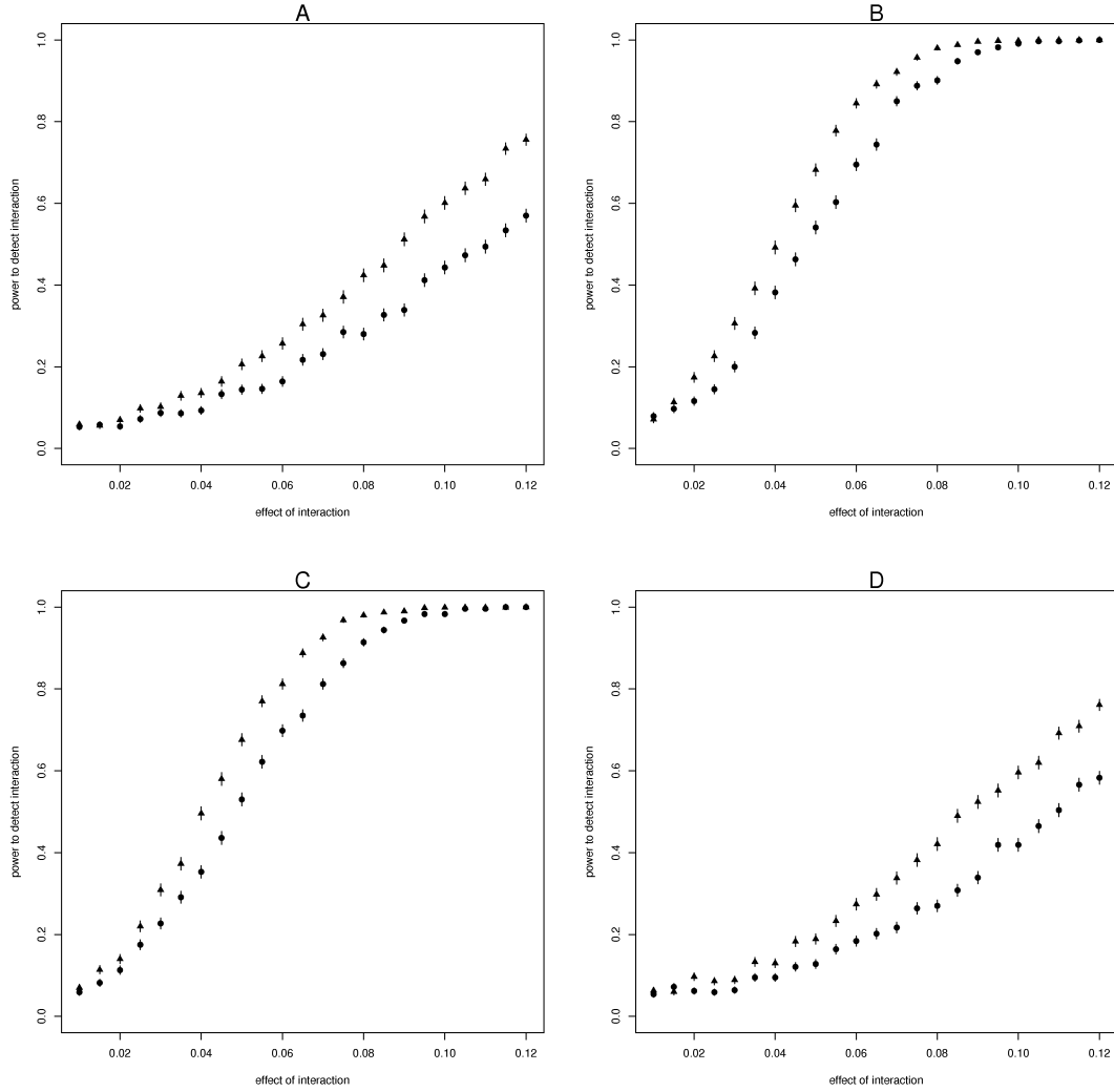
Figure S1: Power to detect variance heterogeneity induced by interaction, assuming Normal distribution of residual error. Dependency of power to detect variance heterogeneity induced by interaction and the effect of interaction, \beta_{gF} , using Levene's (circles) and SVLM (triangles) tests. The residual error follows Normal distribution. Scenarios with different frequencies of interacting allele are given in Panel A – 5%, Panel B – 40%, Panel C – 60%, and Panel D – 95%.
