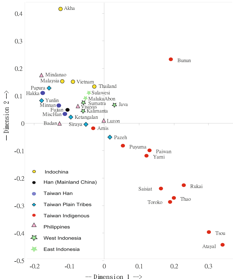
Multiple Dimension Scaling (stress: 0.111)
