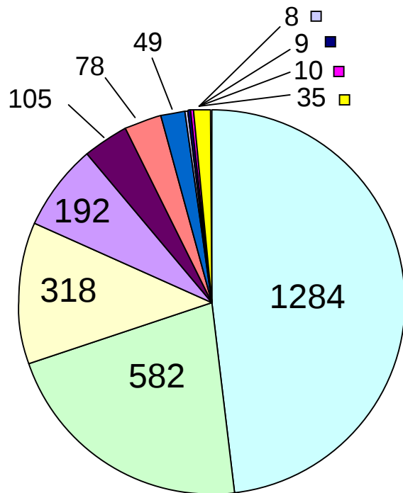
B) Number of sequences (total 2670)
