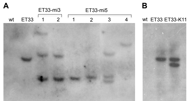
Figure S1 - Evaluation of the Tol2 copy numbers in F 1 fish
