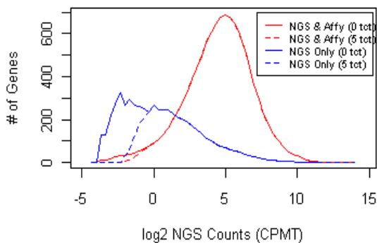
NGS Unique vs NGS and Affy Concordant (HBRR)
