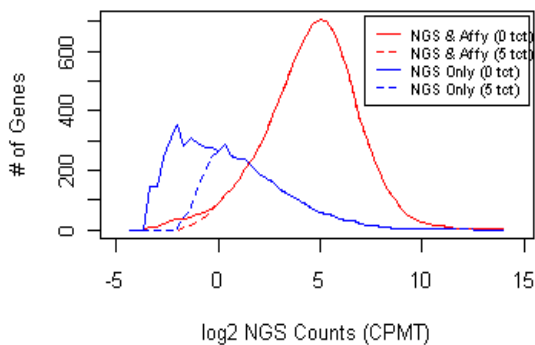
NGS Unique vs NGS and Affy Concordant (UHRR)
