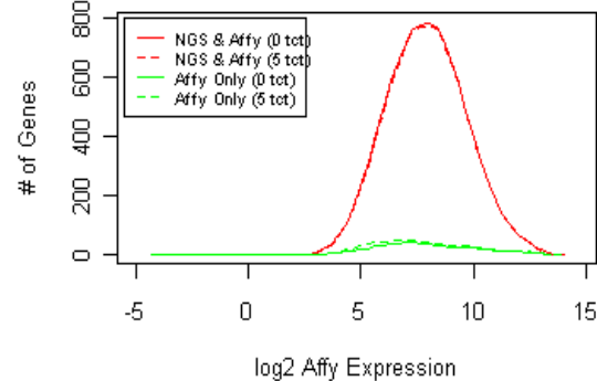
Affy Unique vs NGS and Affy Concordant (HBRR)
