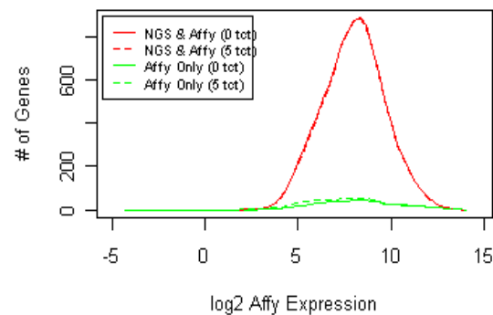
Affy Unique vs NGS and Affy Concordant (UHRR)
