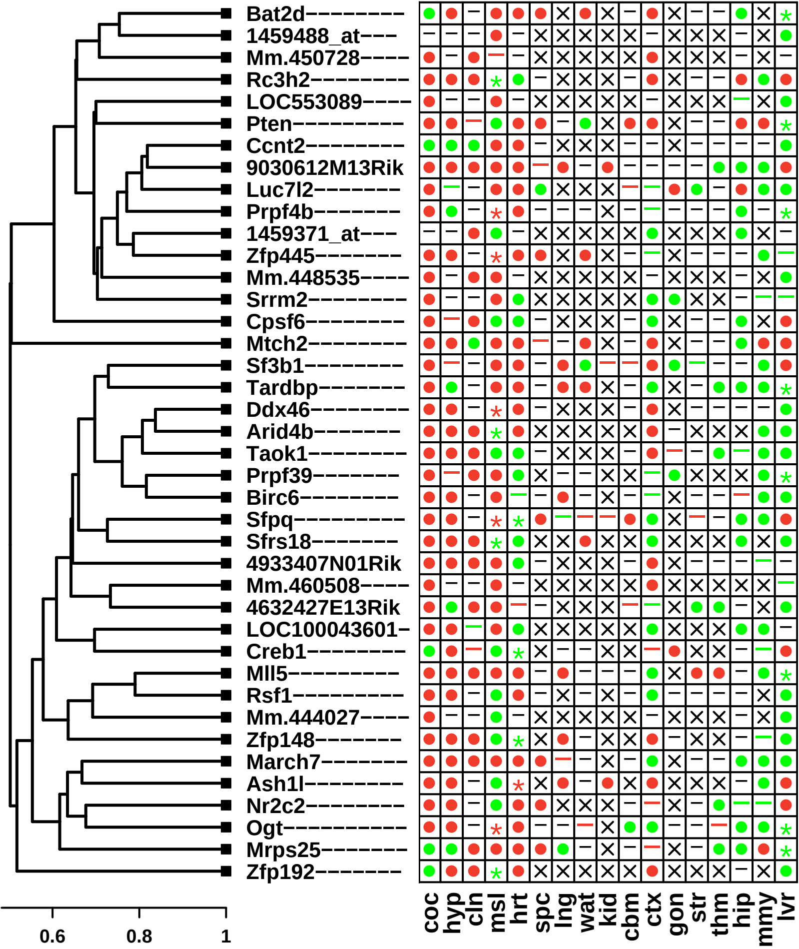
Absolute Correlation
