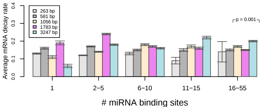
(c) RNA22
