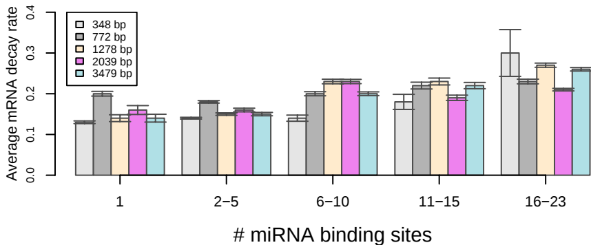
(a) PicTar
