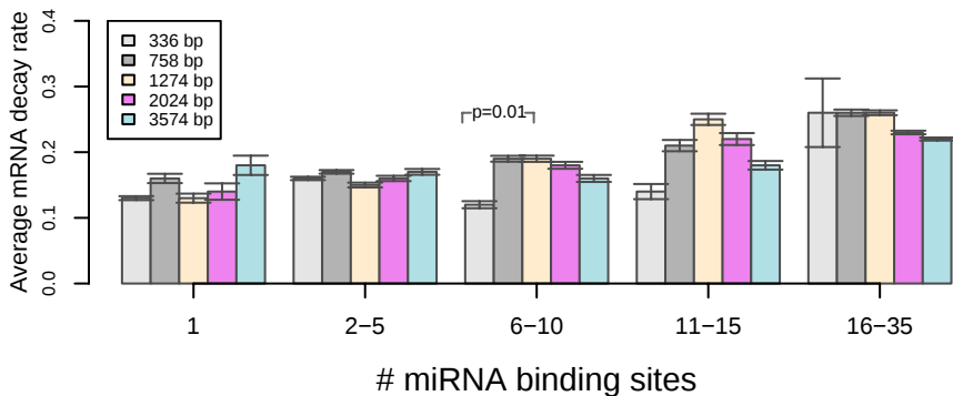
(b) TargetScanS
