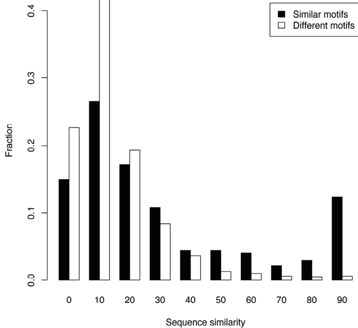
The sequence similarity of neighboring unique genes
