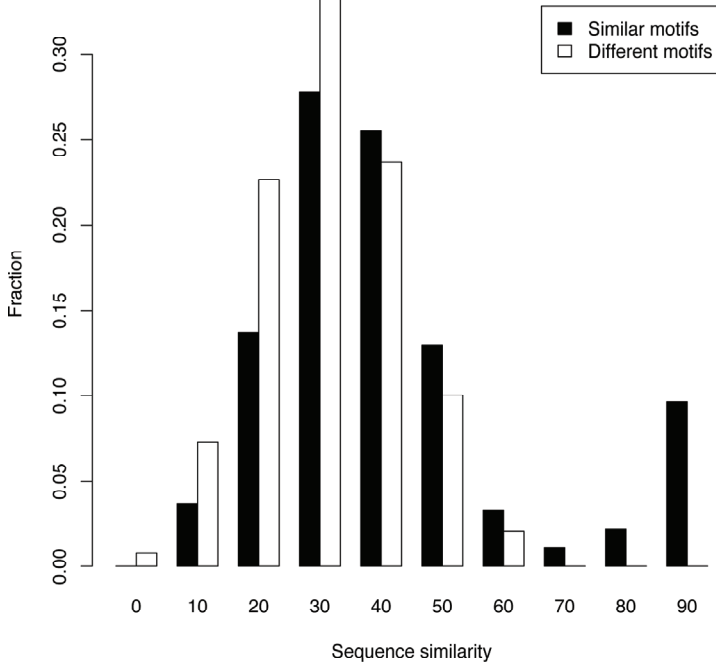
The sequence similarity of neighboring unique core promoters
