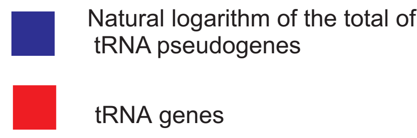
A. Distribution of tRNA gene and tRNA pseudogenes
