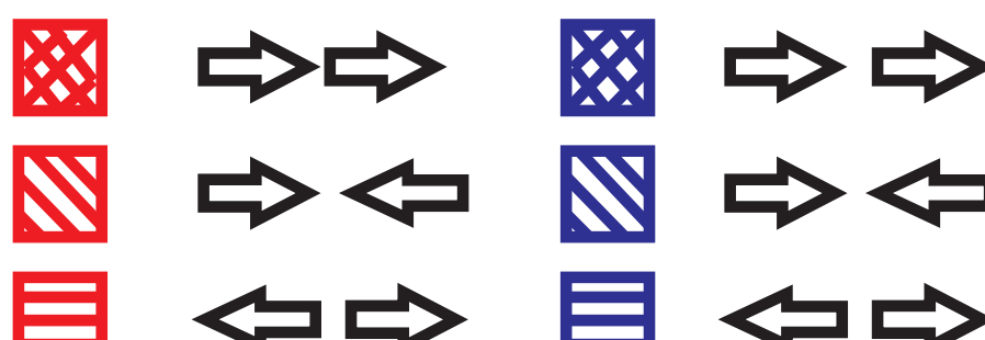
C. Fraction of homogeneous pairs
