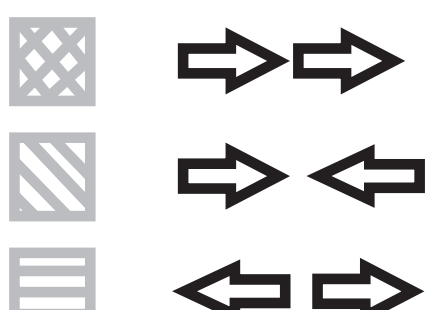
C'. Fraction of heterogeneous pairs
