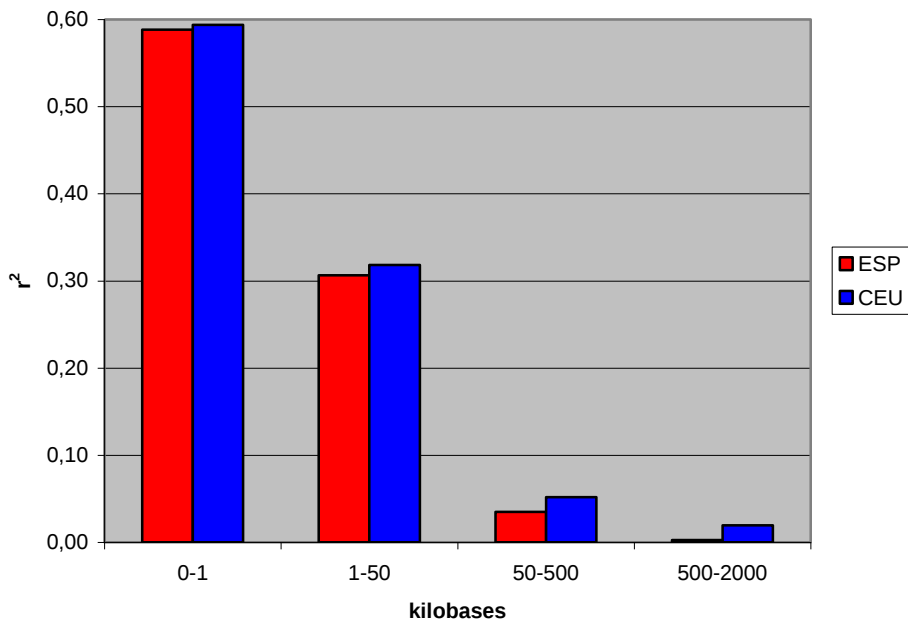
LD Decay ( r^2 )
