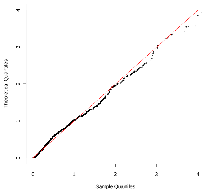
QQ-plot distr. Gamma. Chr-12
