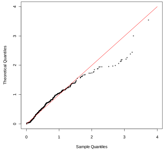
QQ-plot distr. Gamma. Chr-9
