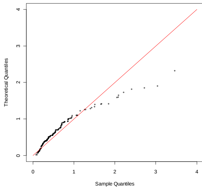
QQ-plot distr. Gamma. Chr-21
