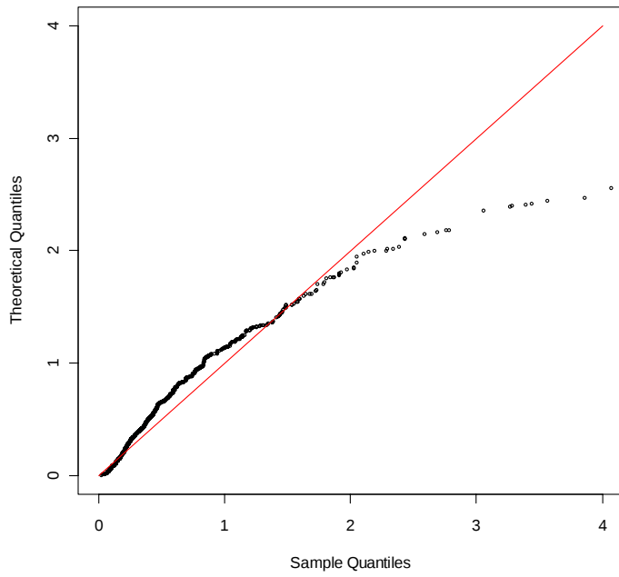
QQ-plot distr. Gamma. Chr-6
