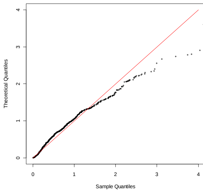
QQ-plot distr. Gamma. Chr-11
