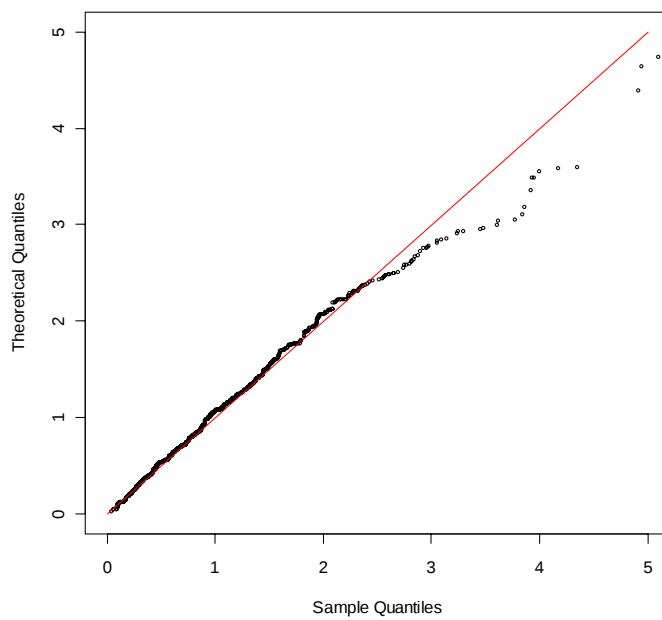
QQ-plot distr. Gamma. Chr-17
