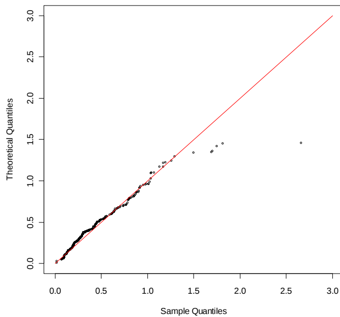
QQ-plot distr. Gamma. Chr-13
