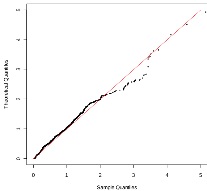
QQ-plot distr. Gamma. Chr-16
