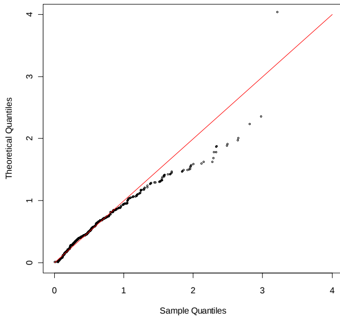
QQ-plot distr. Gamma. Chr-8
