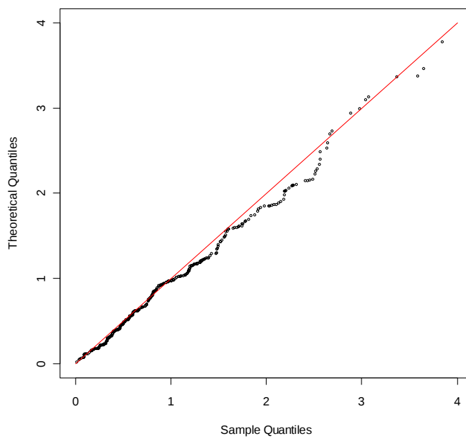
QQ-plot distr. Gamma. Chr-22
