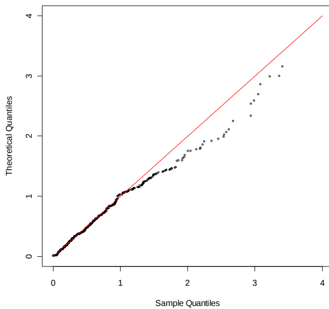
QQ-plot distr. Gamma. Chr-20
