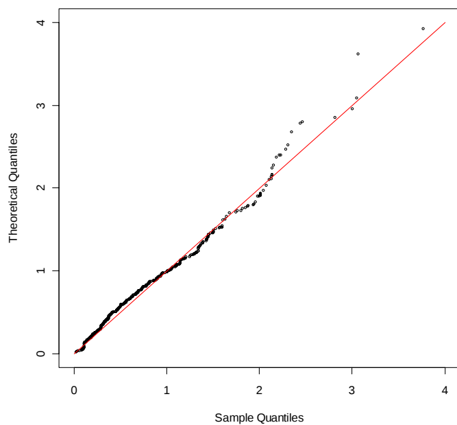
QQ-plot distr. Gamma. Chr-14
