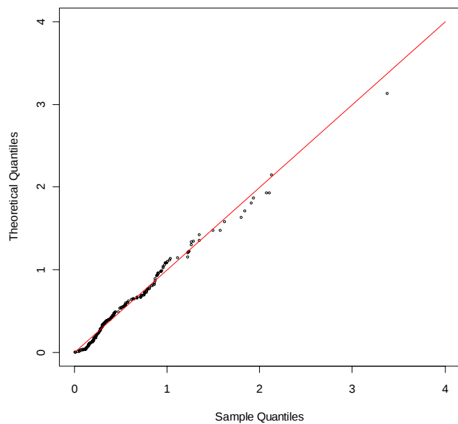
QQ-plot distr. Gamma. Chr-18
