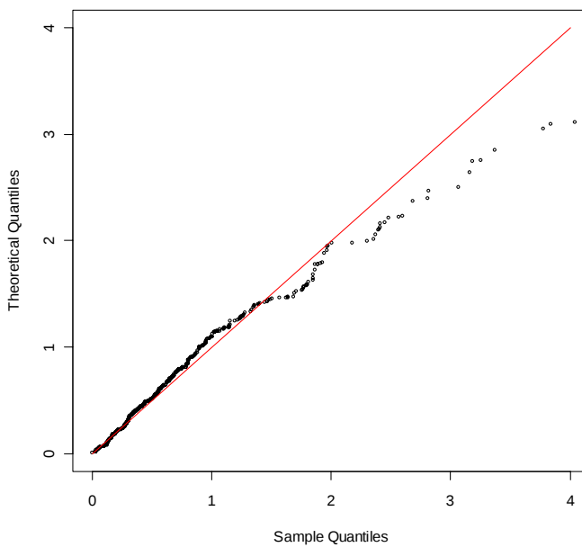
QQ-plot distr. Gamma. Chr-15
