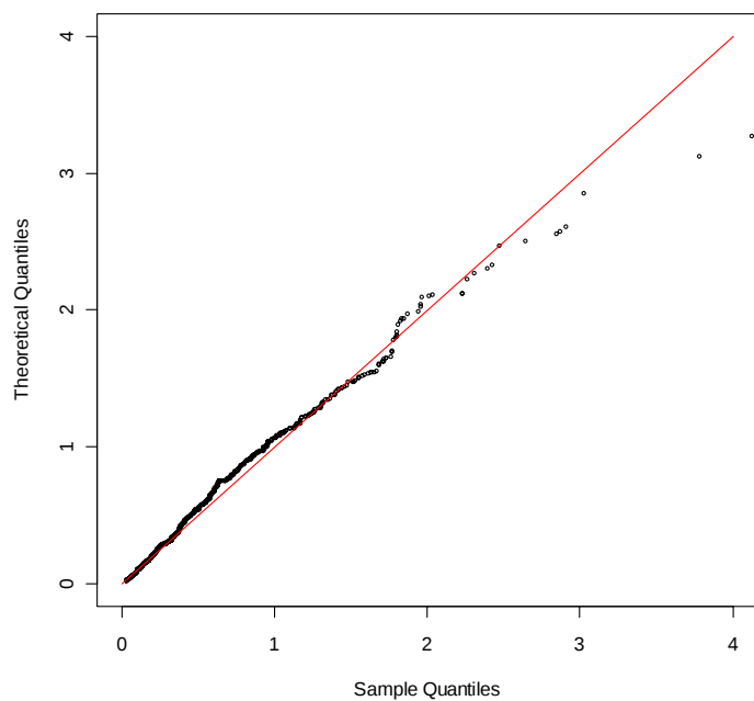
QQ-plot distr. Gamma. Chr-10
