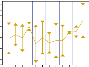
(B) Cidea
