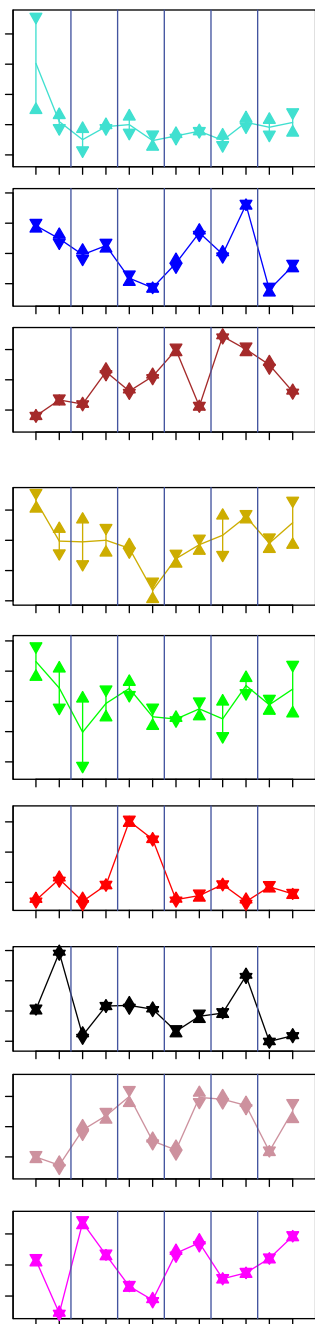
(B) Liver Affymetrix
