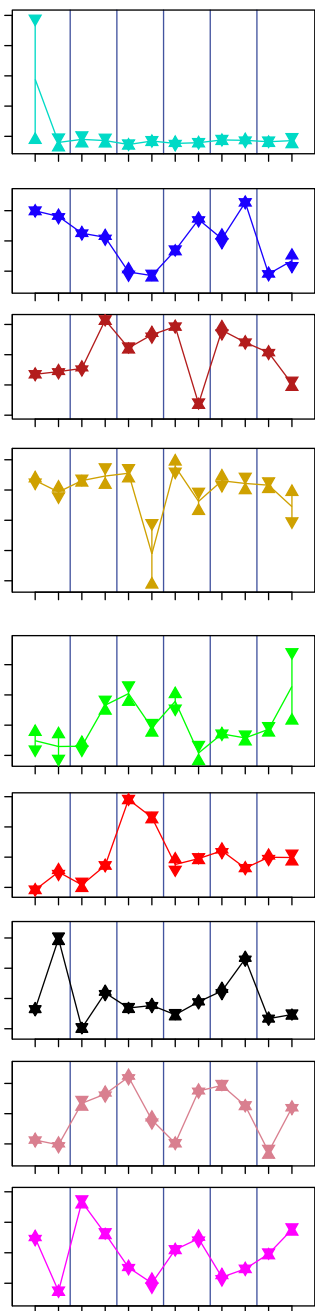
(A) Liver Illumina
