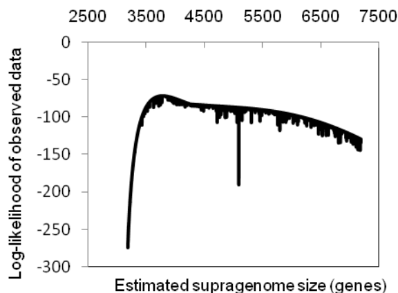
Streptococcus pneumoniae (17 strains) [ supragenome estimate 3783 genes ]
