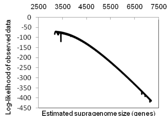
Staphylococcus aureus (17 strains) [ supragenome estimate 3221 genes ]
