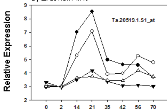
C) Extensin-like
