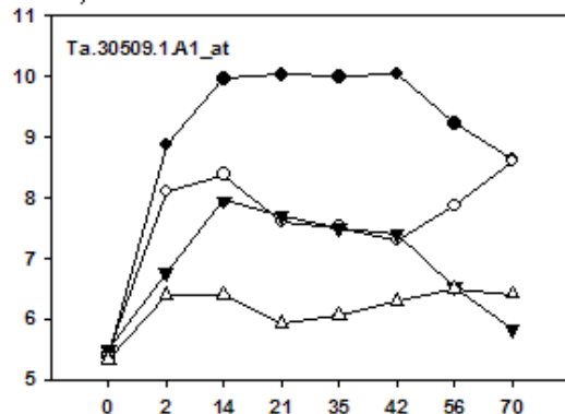
D) Protamine
