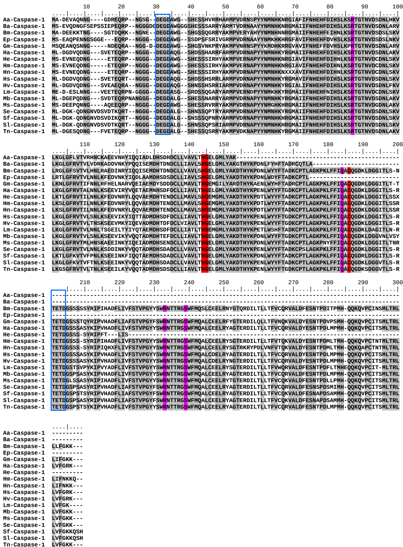
Figure S1. Amino acid alignment of Lep-Caspase-1 sequences. Identical residues are boxed in grey. Critical amino acids involved in substrate-binding are boxed in purple. Critical amino acids involved in the active site, including the catalytic cysteine residue, are boxed in red. Blue frames indicate cleavage sites.
