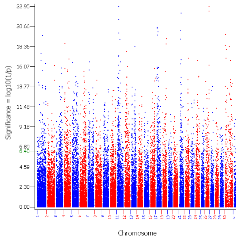
Manhattan Plot: TL
