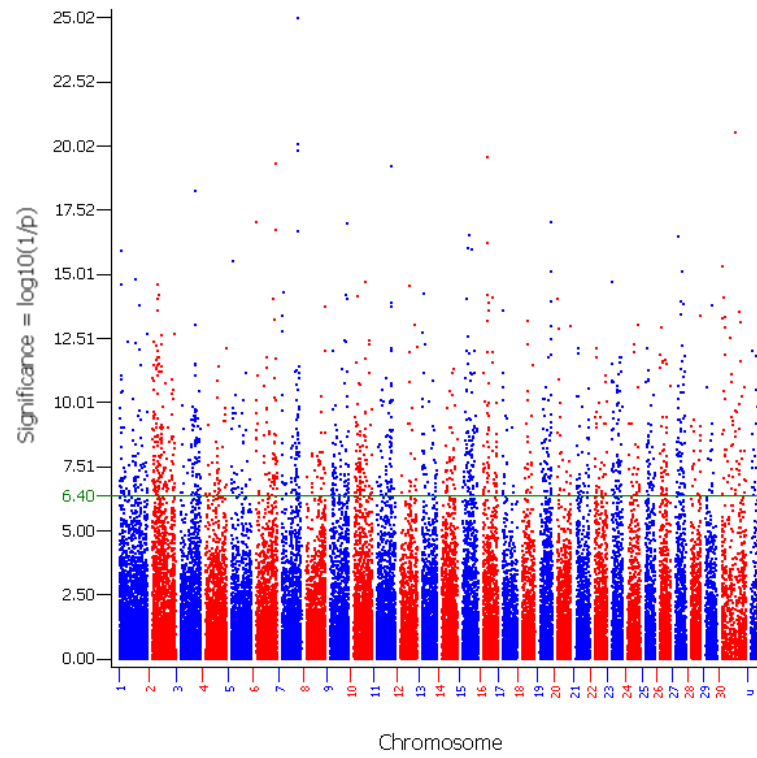
Manhattan Plot: RTP
