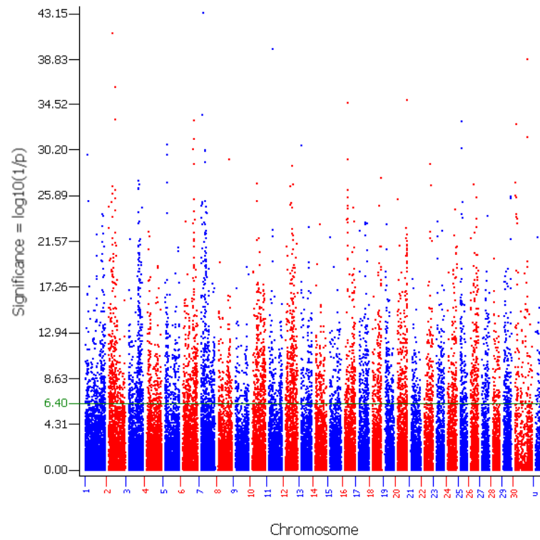
Manhattan Plot: SCS
