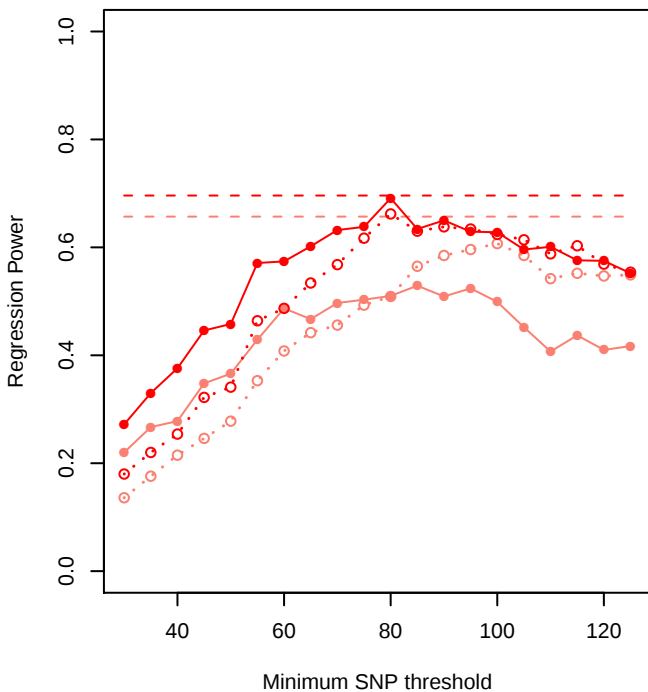
PLINK light LD-pruning Autozygosity within 20 generations
