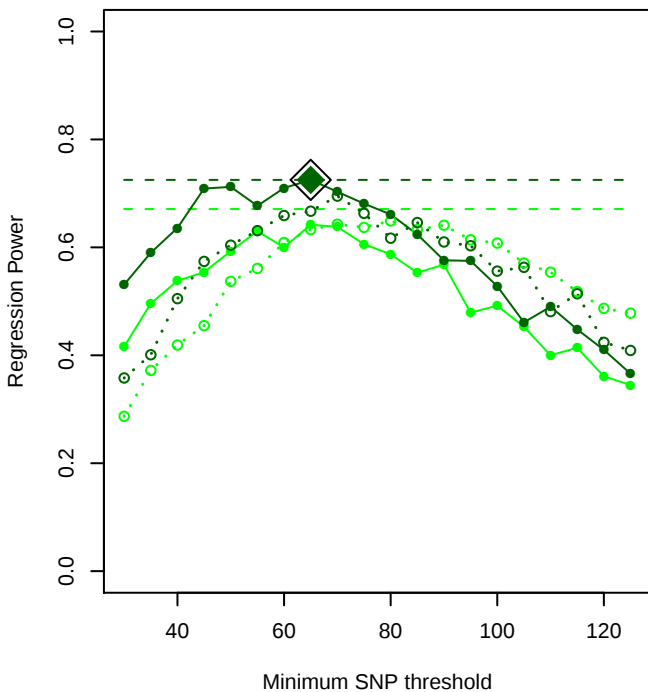
Autozygosity within 50 generations
