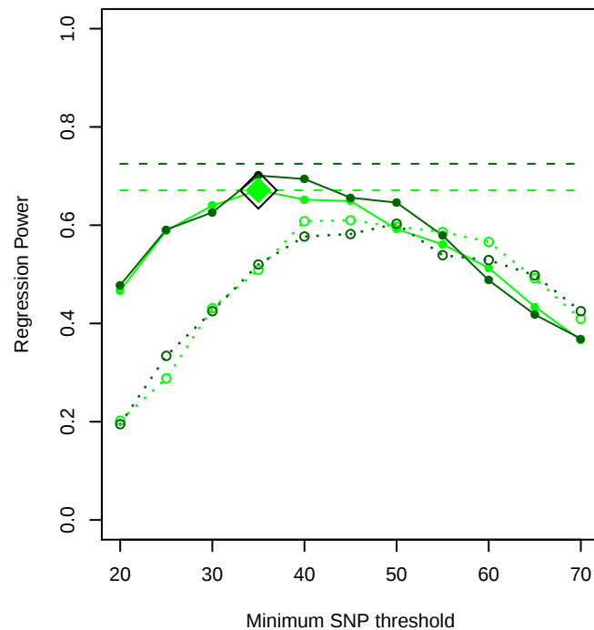
Autozygosity within 50 generations
