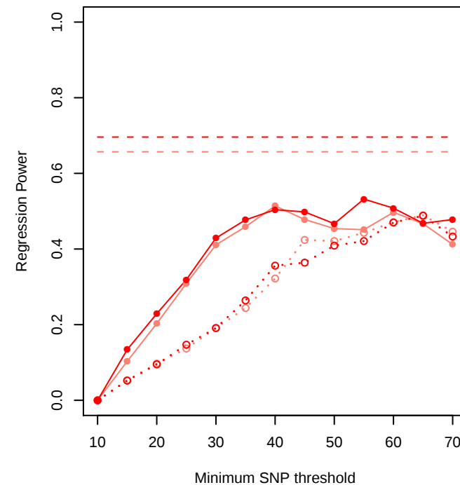
PLINK moderate-heavy LD-pruning Autozygosity within 20 generations
