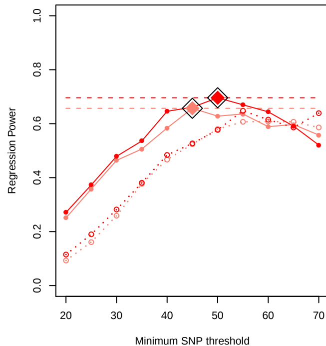
PLINK moderate LD-pruning Autozygosity within 20 generations
