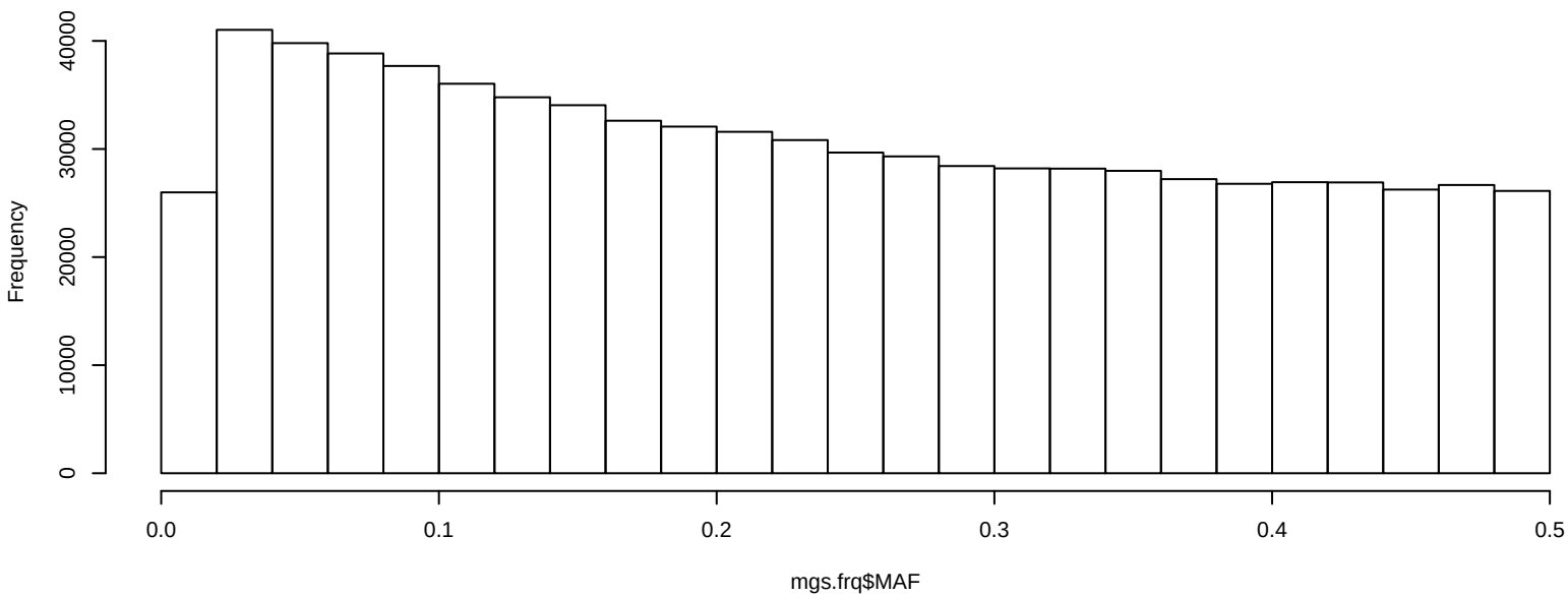
MAF distribution in MGS control data
