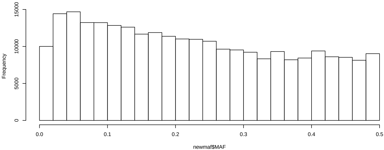
MAF distribution in Sequence data after pruning for MAF
