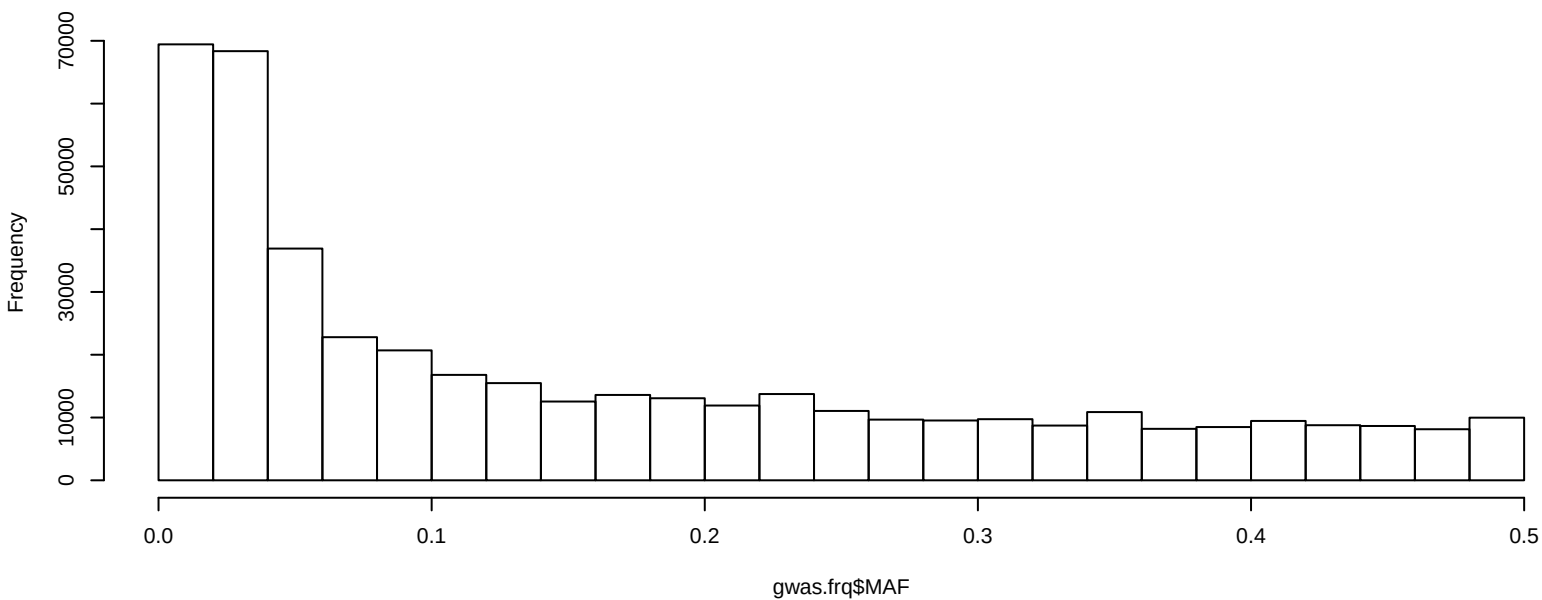
MAF distribution in Sequence Data (no MAF<.01)
