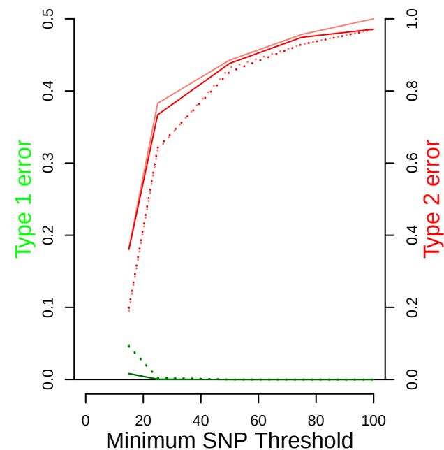
PLINK – hvypruned SNP data
