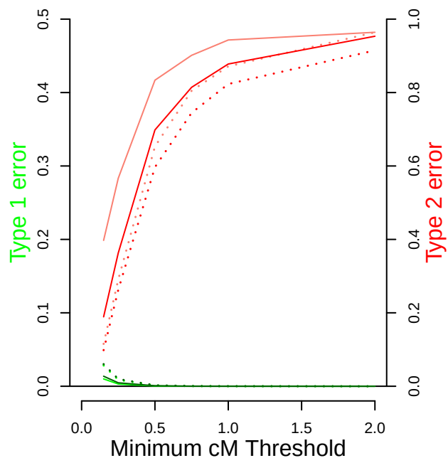
GERMLINE – unpruned SNP data
