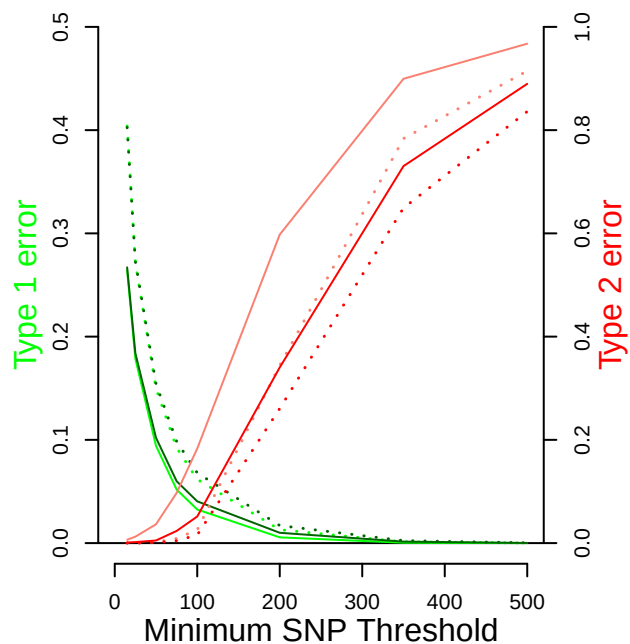
PLINK – unpruned SNP data
