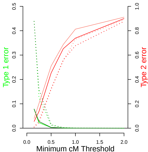
GERMLINE – modpruned SNP data
