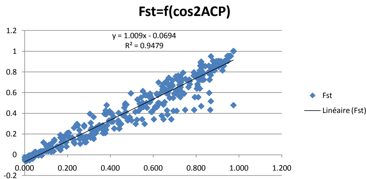
Figure A1: Correlation between the contribution of SNPs loci to the first axis of PCA analysis ( C. maxima and C. reticulata as active individuals) and the F_{st} values for C. maxima / C. reticulata differentiation
