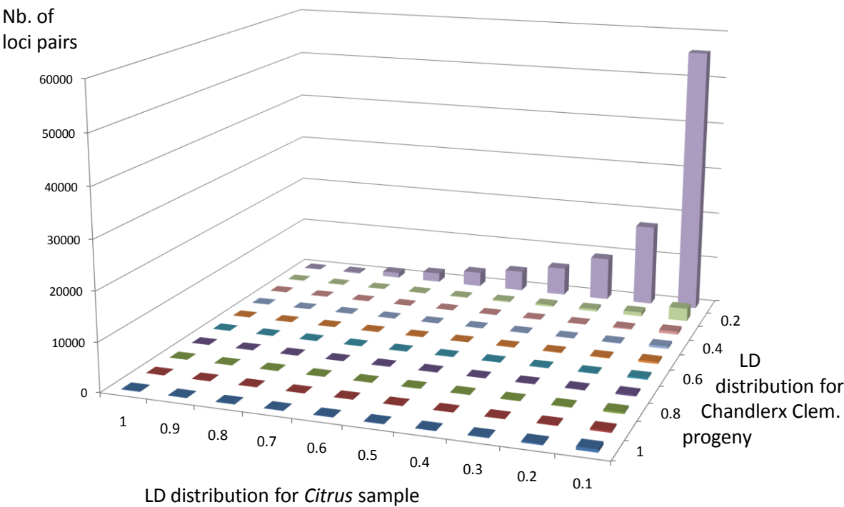
Figure A2: Co-distribution of Linkage Disequilibrium (LD estimated by r^2 ) between WONA locus pairs for Chandler x Clementine progeny and germplasm population.
