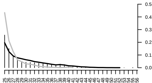
Read length
