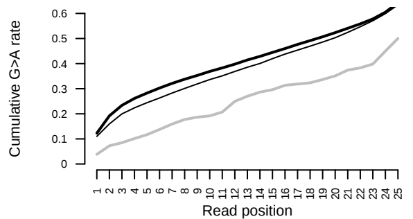
Read position
