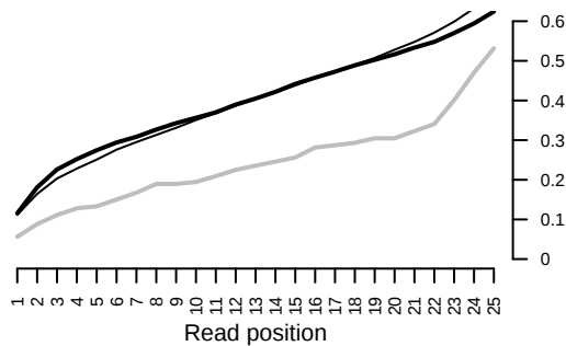
Read position
