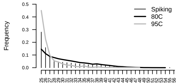
Read length
